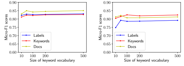
(a) WESTCLASS-CNN
