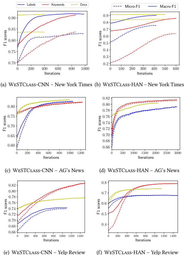
Figure 2: Effect of self-training modules on three datasets.
