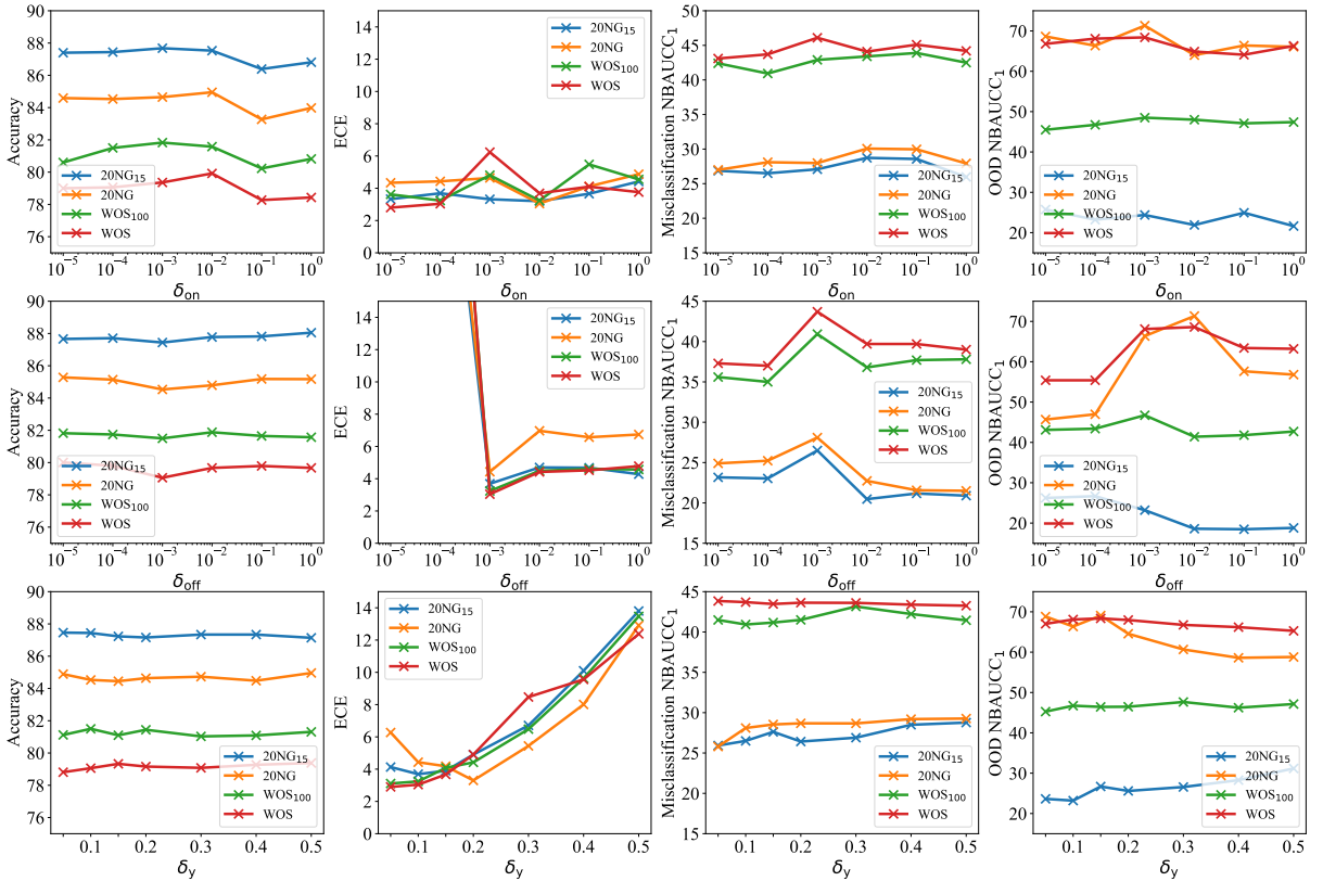
Figure 5: Parameter study of \delta_{\text{on}} , \delta_{\text{off}} and \delta_y . We use NBAUC 1 for OOD and misclassification detection.
